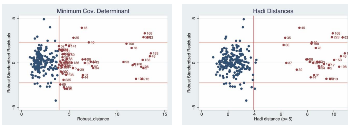
Figure 5 - Outliers identified with robust estimators.
