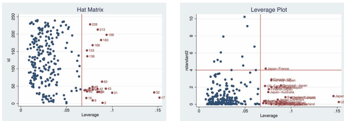
Figure 1 - Outliers: Hat Matrix and Leverage Plot.
